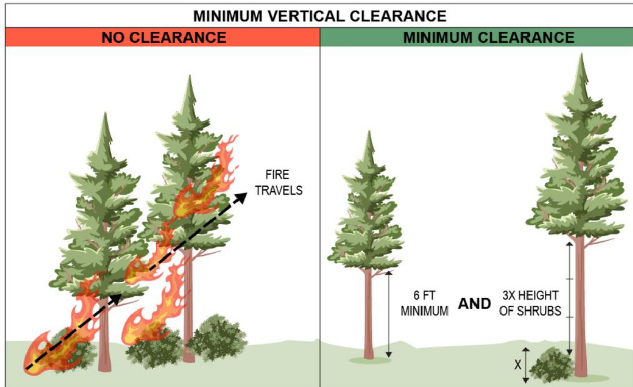
Figure 7.4.2: Vertical Spacing
